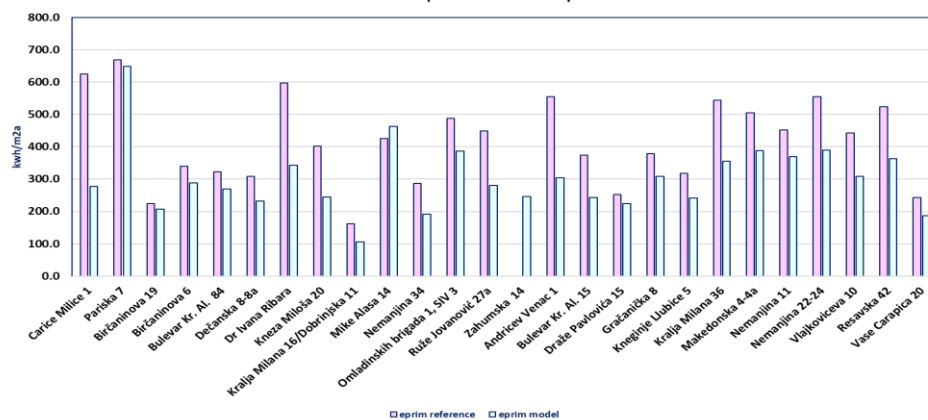
Specific annual primary energy reference eprim vs modelled eprim
